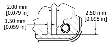
DETAIL U
