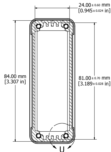
SECTION T-T
