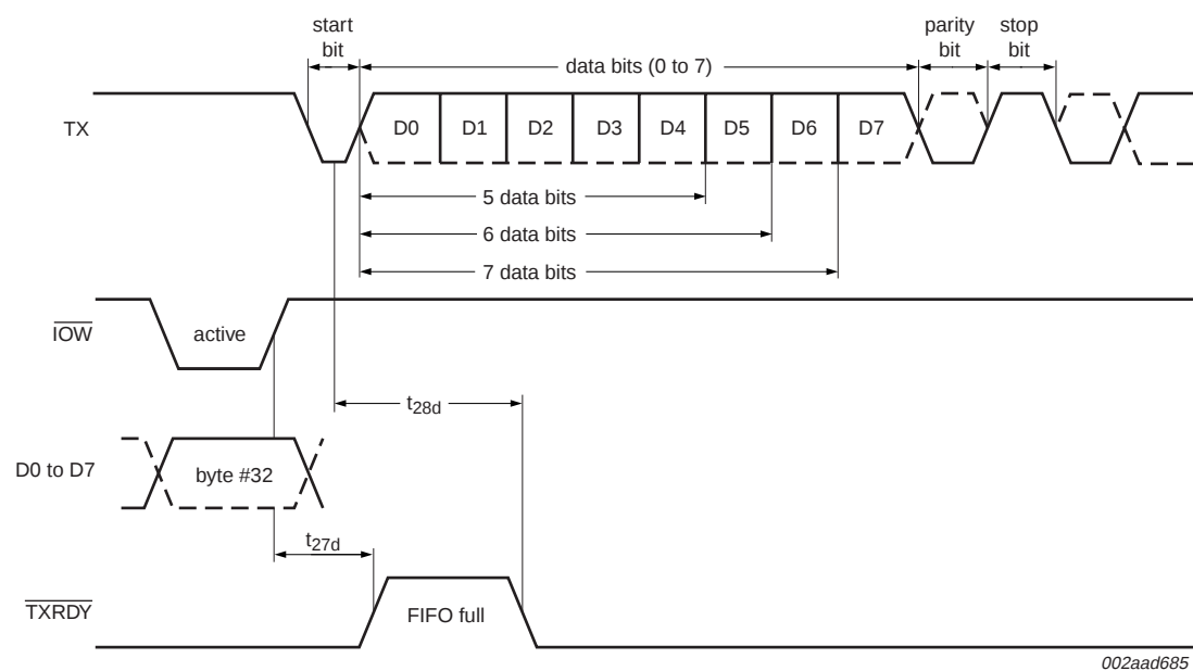
Fig 19. Transmit ready timing in FIFO mode (DMA mode '1')
