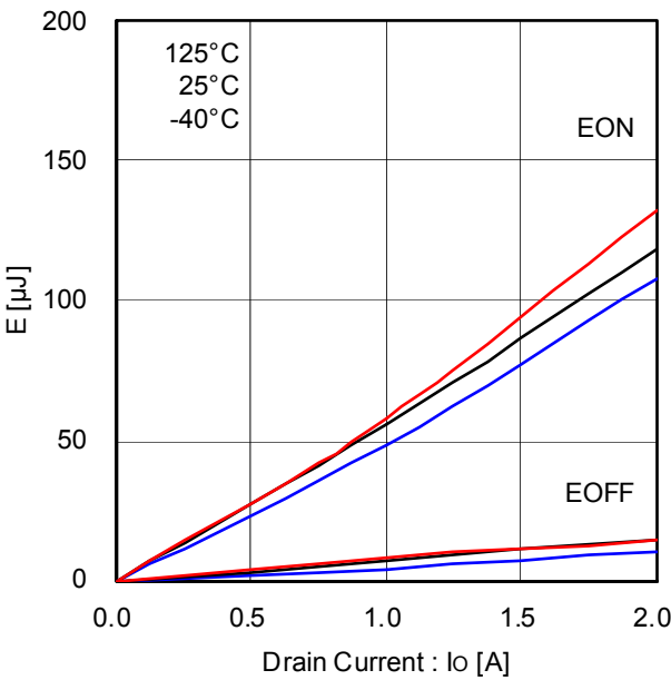
Figure 25. Low Side Switching Loss (VDC=150V)
