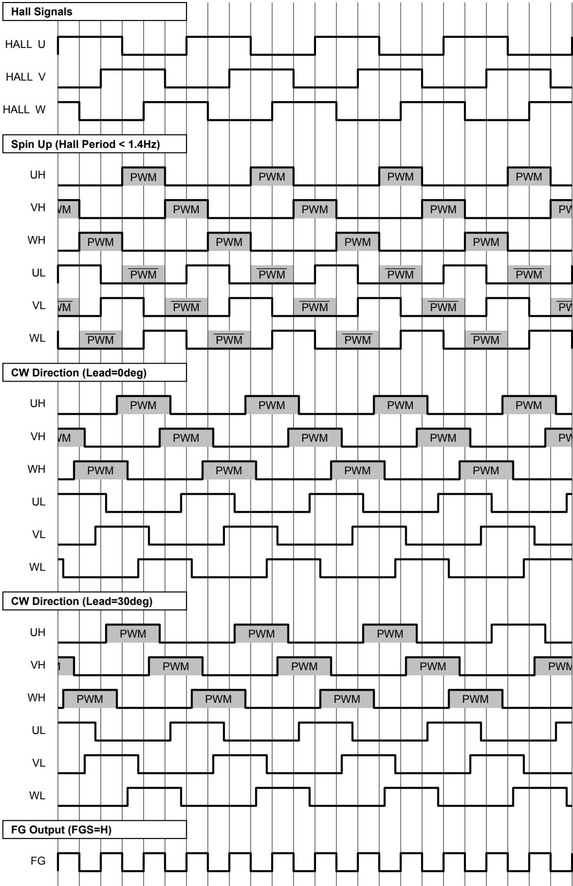
Timing Chart (CW)
