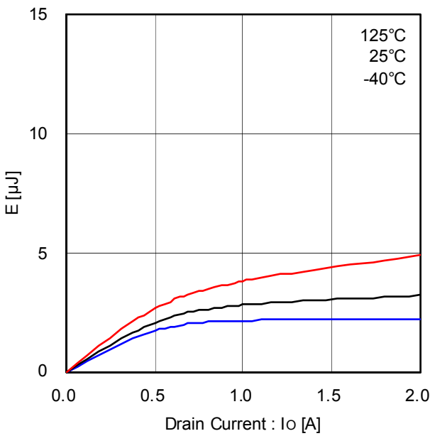
Figure 24. High Side Recovery Loss (VDC=150V)
