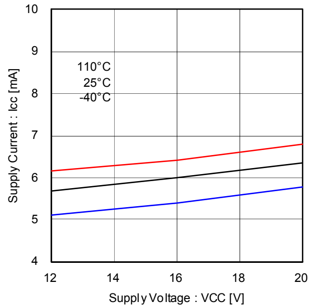
Figure 16. Low Side Drivers Operating Current ( F_{PWM} : 20kHz)
