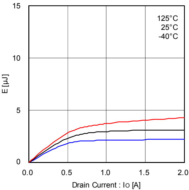
Figure 26. Low Side Recovery Loss (VDC=150V)
