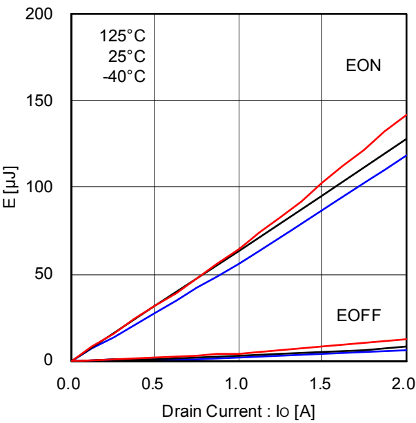
Figure 23. High Side Switching Loss (VDC=150V)
