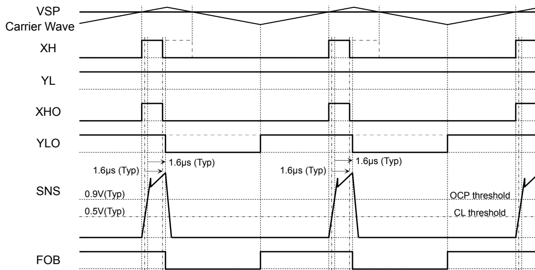
Figure 9. Fault Operation ~ OCP ~ Timing Chart
