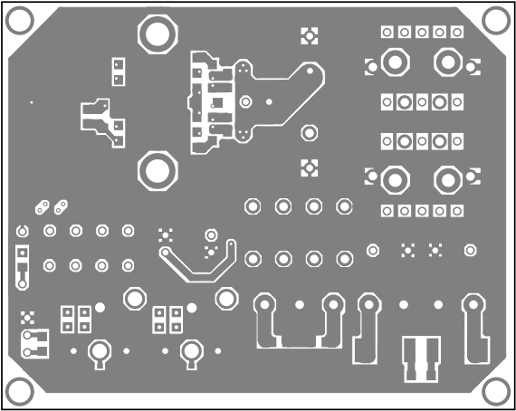
Bottom copper
