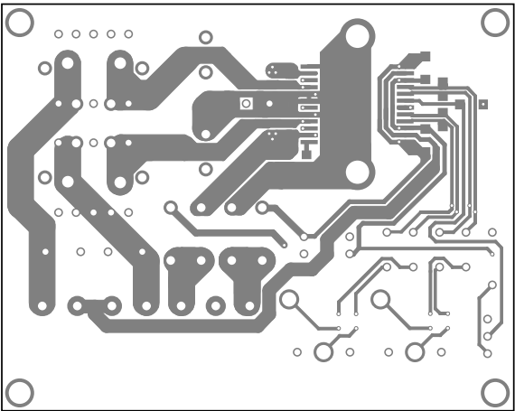
Top copper
