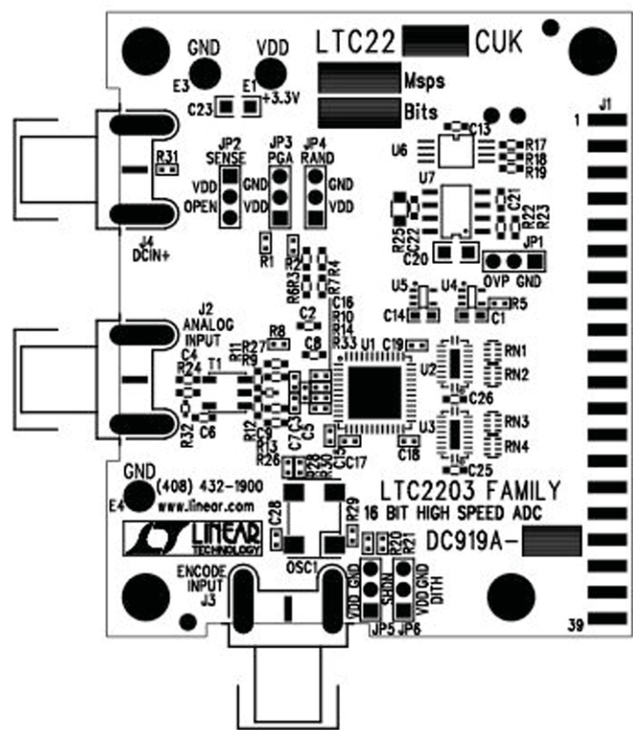
Silkscreen Top
