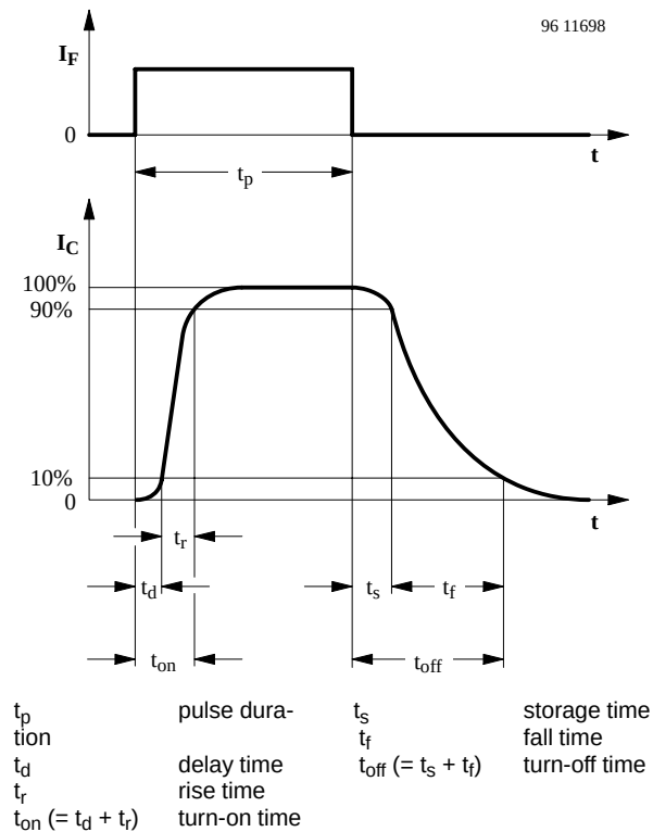
Figure 3. Switching times
