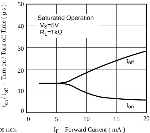
95 11031 I_F – Forward Current ( mA ) Figure 12. Turn on / off Time vs. Forward Current
