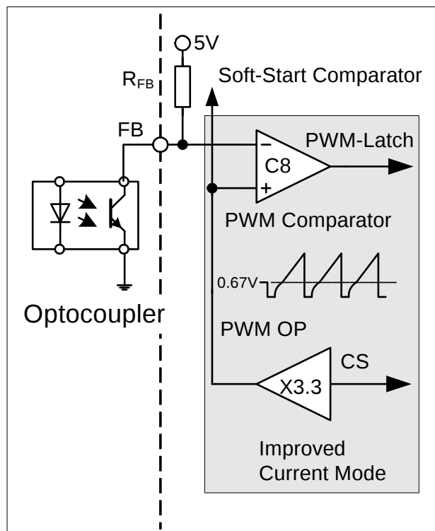
Figure 8 PWM Controlling
