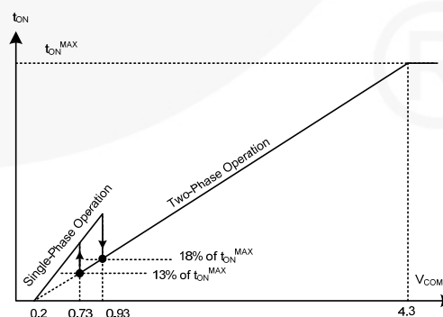
Figure 30. V_{COMP} vs. t_{ON}^{MAX}
