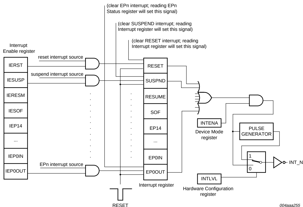
Fig 8. Interrupt logic
