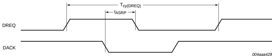
Fig 19. DMA timing in 8237 compatible mode
