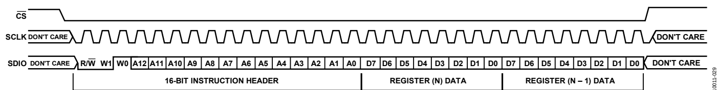
Figure 28. Serial Control Port Write—MSB First, 16-Bit Instruction, Two Bytes of Data
