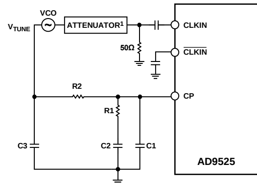
Figure 19. CLKIN Configured as Single-Ended VCO
