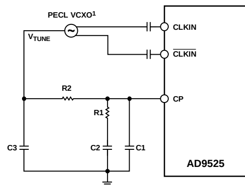
Figure 21. CLKIN Configured as Differential LVPECL VCXO
