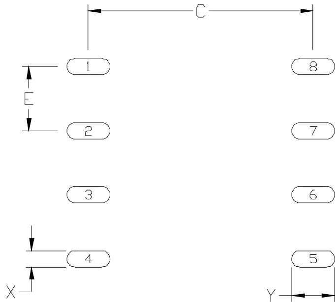
Figure 20. DIP8 Land Pattern
