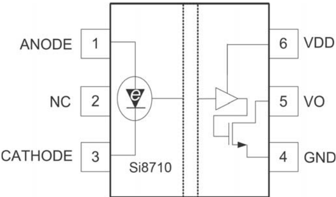
Figure 15. Pin Configuration
