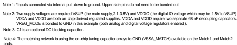
Figure 5-2 • ZL70101 Transceiver Configured for an Implant – Optimal Performance
