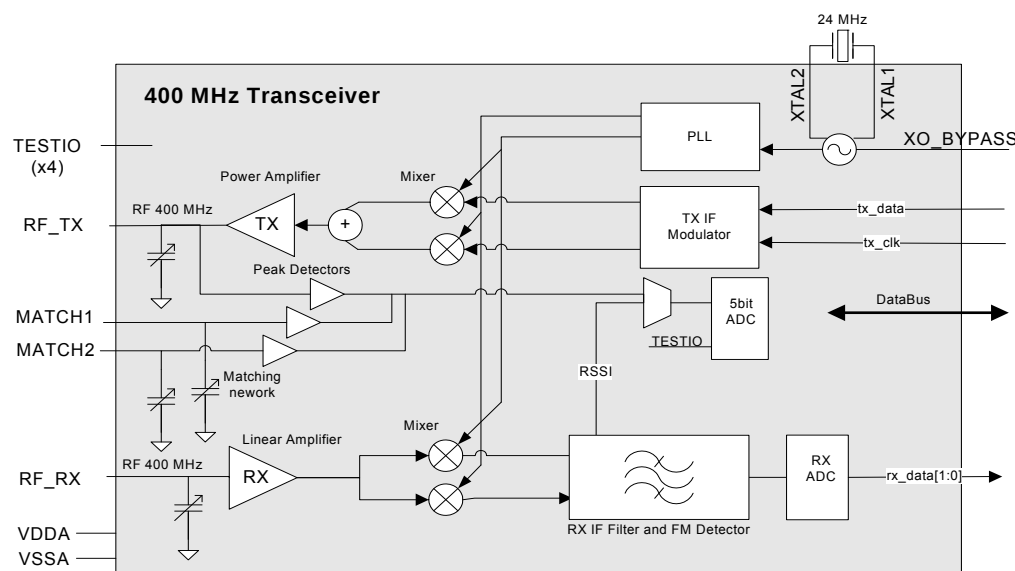
Figure 1-3 • 400 MHz Transceiver Subsystem
