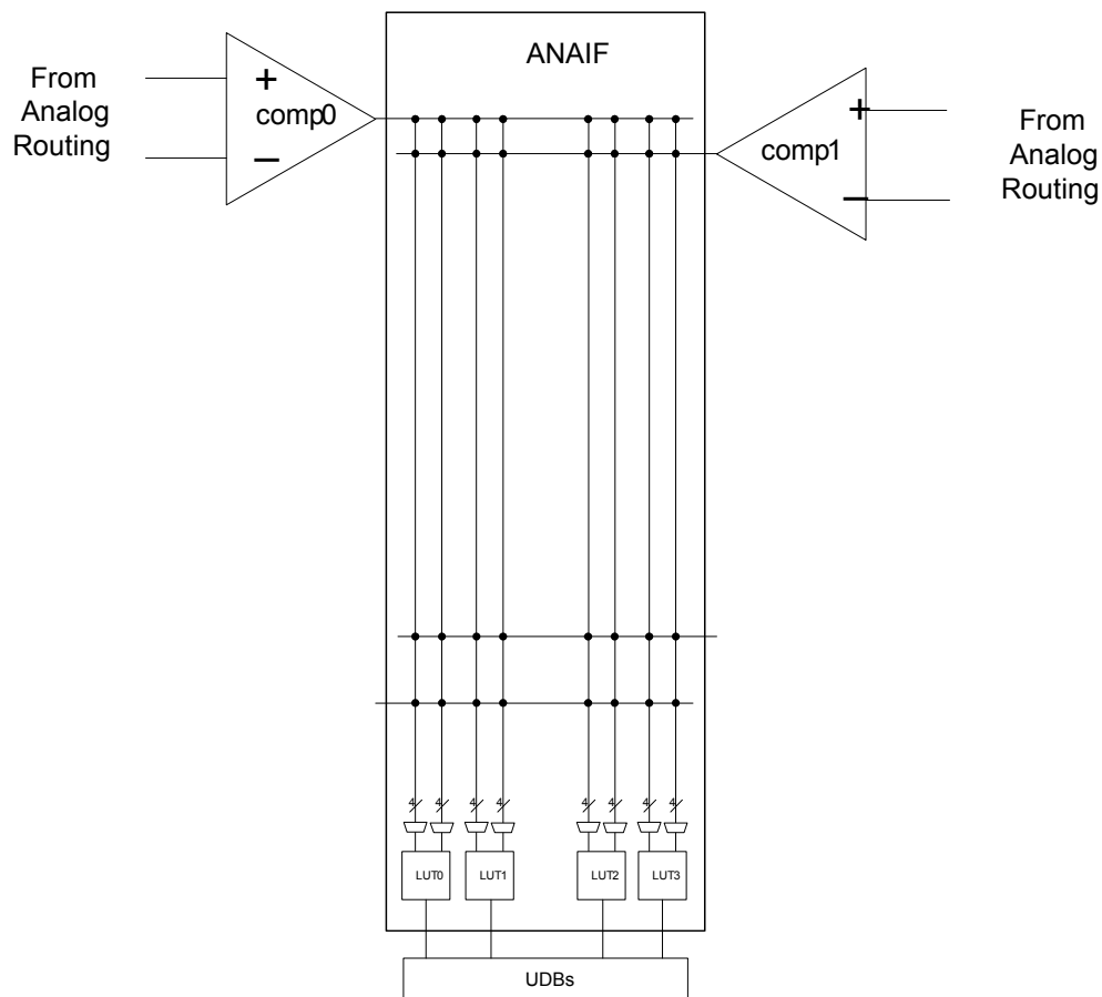
Figure 8-5. Analog Comparator
