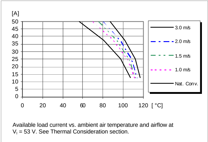
Output Current Derating – Open frame
