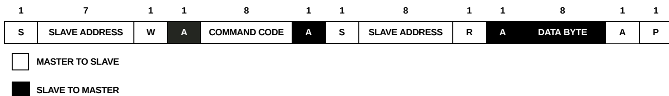
FIGURE 30. READ BYTE PROTOCOL for ISL97694A
