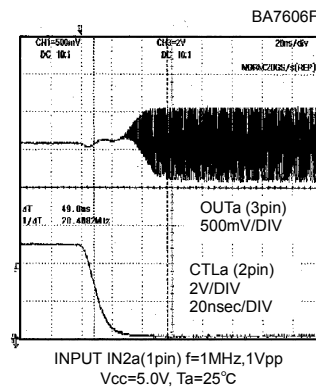
Fig.12 Switching characteristics1 OFF→ON
