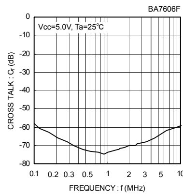
Fig.11 Interchannel crosstalk
