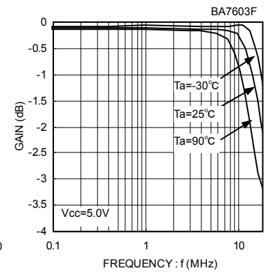
Fig.10 Frequency characteristics vs. temperature
