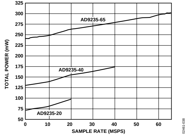
Figure 38. Total Power vs. Sample Rate with f_{\text{IN}} = 10 MHz
