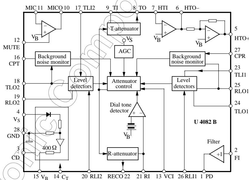
Figure 1. Block diagram
