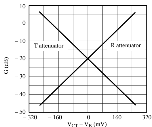
Figure 11. Attenuator gain versus VCT (Pin 14)
