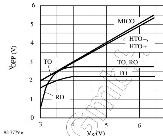
Figure 23. Typical output swing versus V_S
