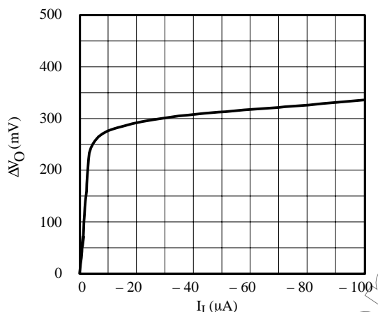
Figure 12. Level detector DC transfer characteristics
