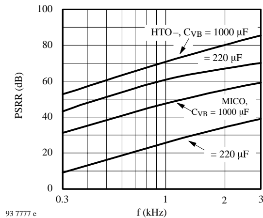
Figure 22. V_B power supply rejection of the microphone and hybrid amplifiers
