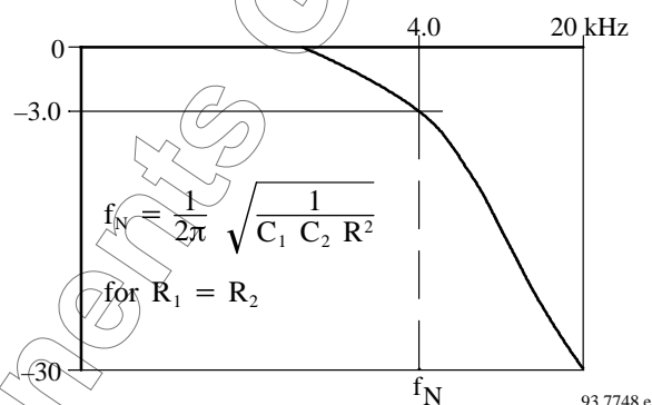
Figure 9. Low-pass filter
