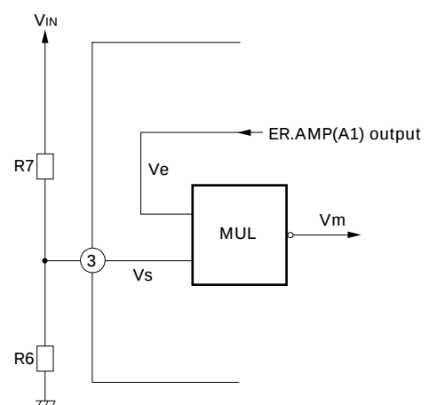
Fig. 6 Multiplier
