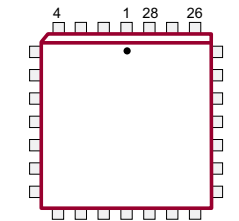
28-Lead PLCC (PJ) (top view)
