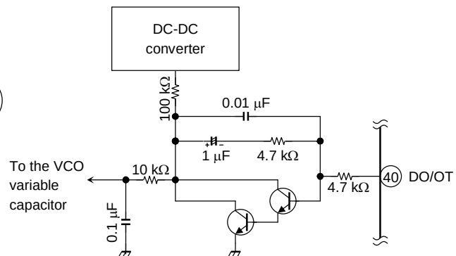
Example of an active low pass filter circuit (for reference)
