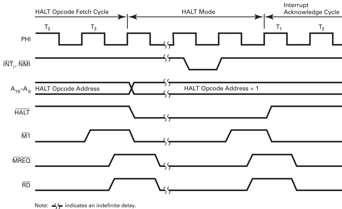
Figure 13. HALT Timing
