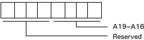
Figure 67. DMA Memory Address Register, Channel 1B
