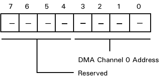
Figure 57. DMA Source Address Register 0B
