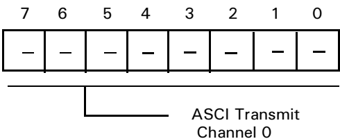
Figure 36. ASCII Register
