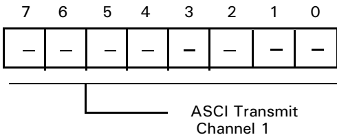
Figure 37. ASCII Register
