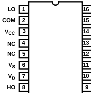
HIP2500 (SOIC) TOP VIEW
