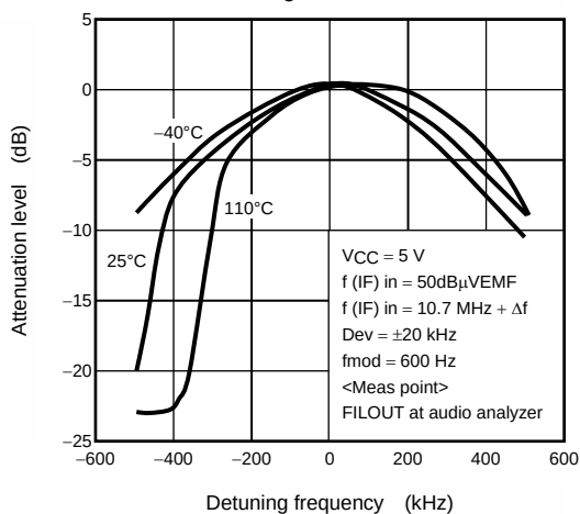
Detuning Characteristics
