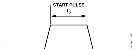
Figure 3. Daisy-Chain Start Timing
