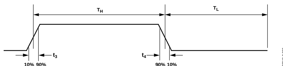
Figure 2. PWM Output Nominal Timing Diagram (25°C)
