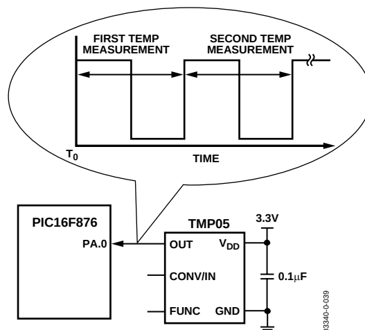
Figure 37. Typical Daisy-Chain Application Circuit
