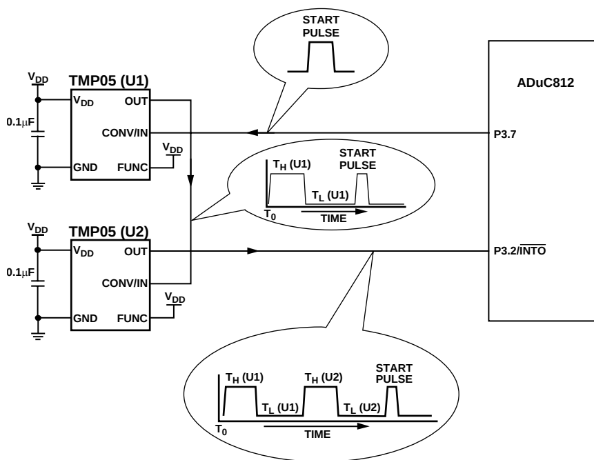
Figure 33. Typical Daisy-Chain Application Circuit
