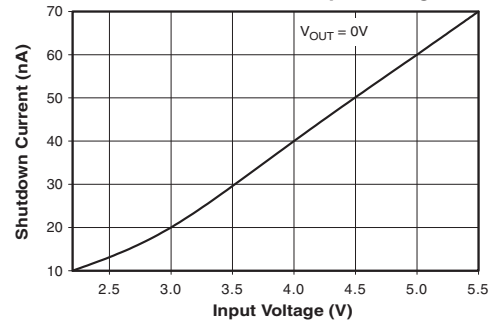
Shutdown Current vs Input Voltage
