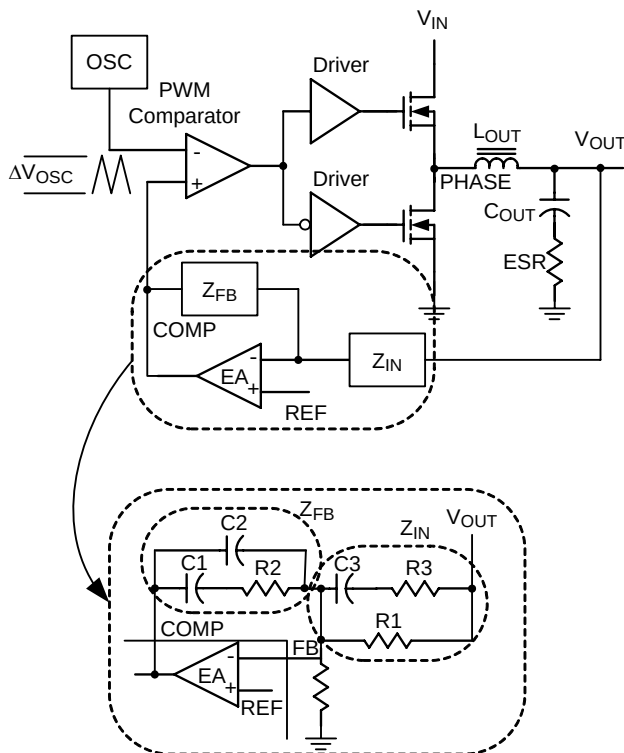
Figure 5. Closed Loop
