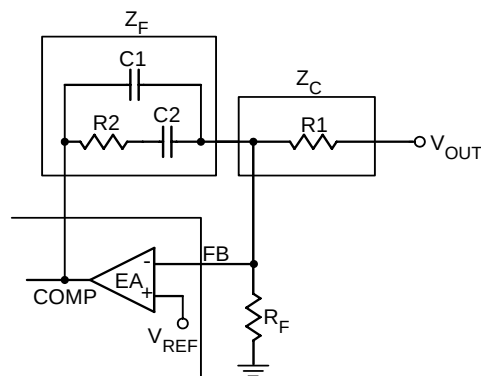
Figure 6. Compensation Loop
