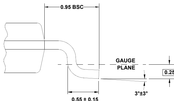
DETAIL "X"
