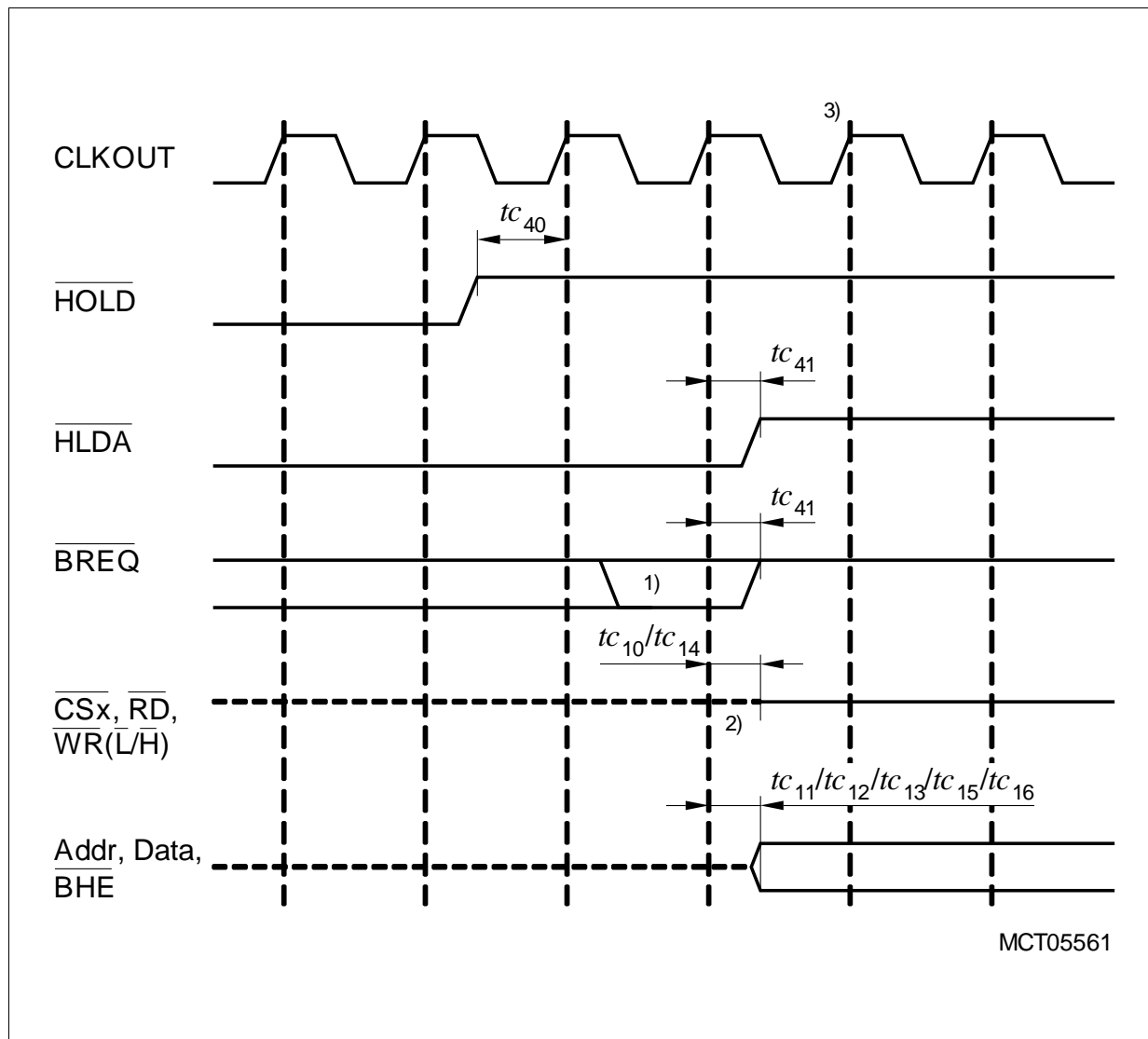
Figure 24 External Bus Arbitration, Regaining the Bus
