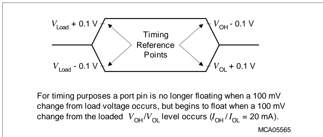
Figure 18 Float Waveforms
