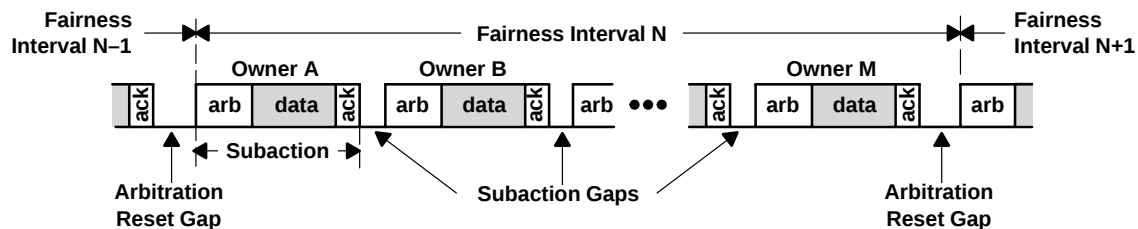
Figure 6–9. Fairness Interval
