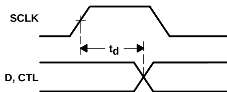
Figure 4–1. Parameter Measurement Information
