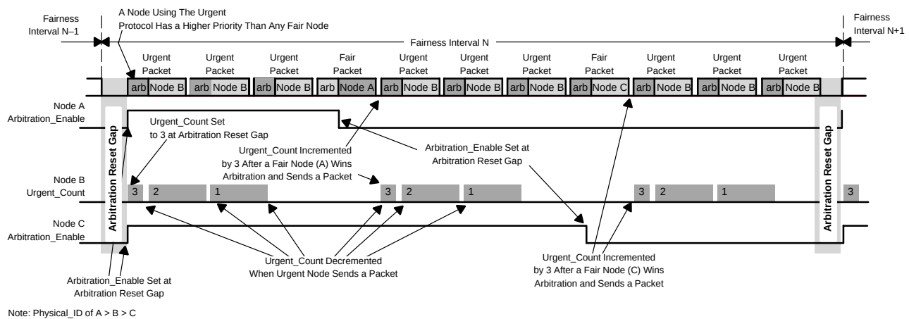
Figure 6–11. Urgent Arbitration
