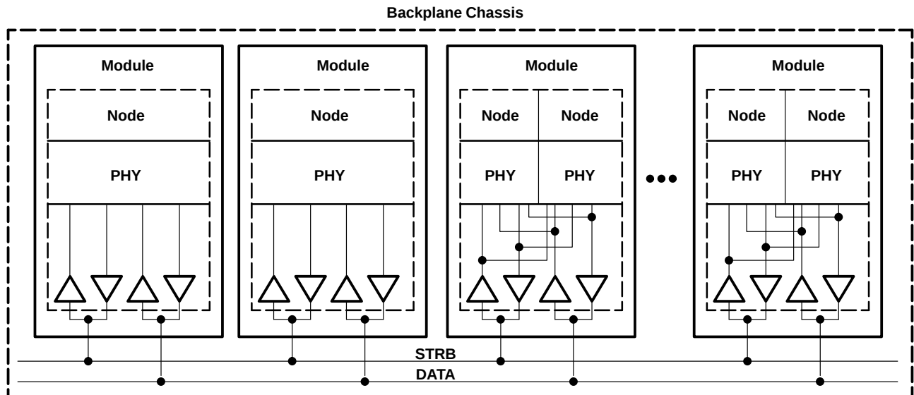
Figure 6–6. Backplane Topology
