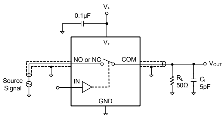
Test Circuit 9. -3dB Bandwidth
