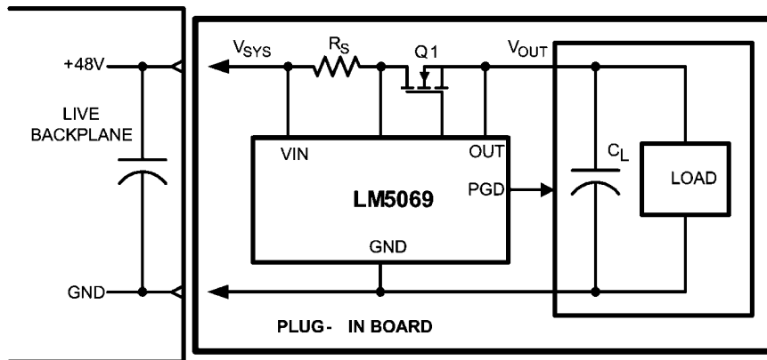
FIGURE 2. LM5069 Application
