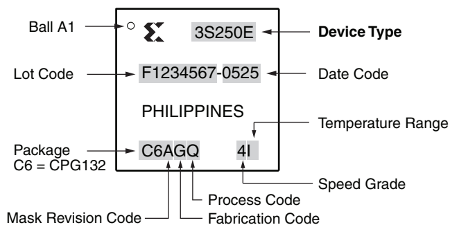
Figure 4: XA Spartan-3E FPGA CPG132 Package Marking Example
