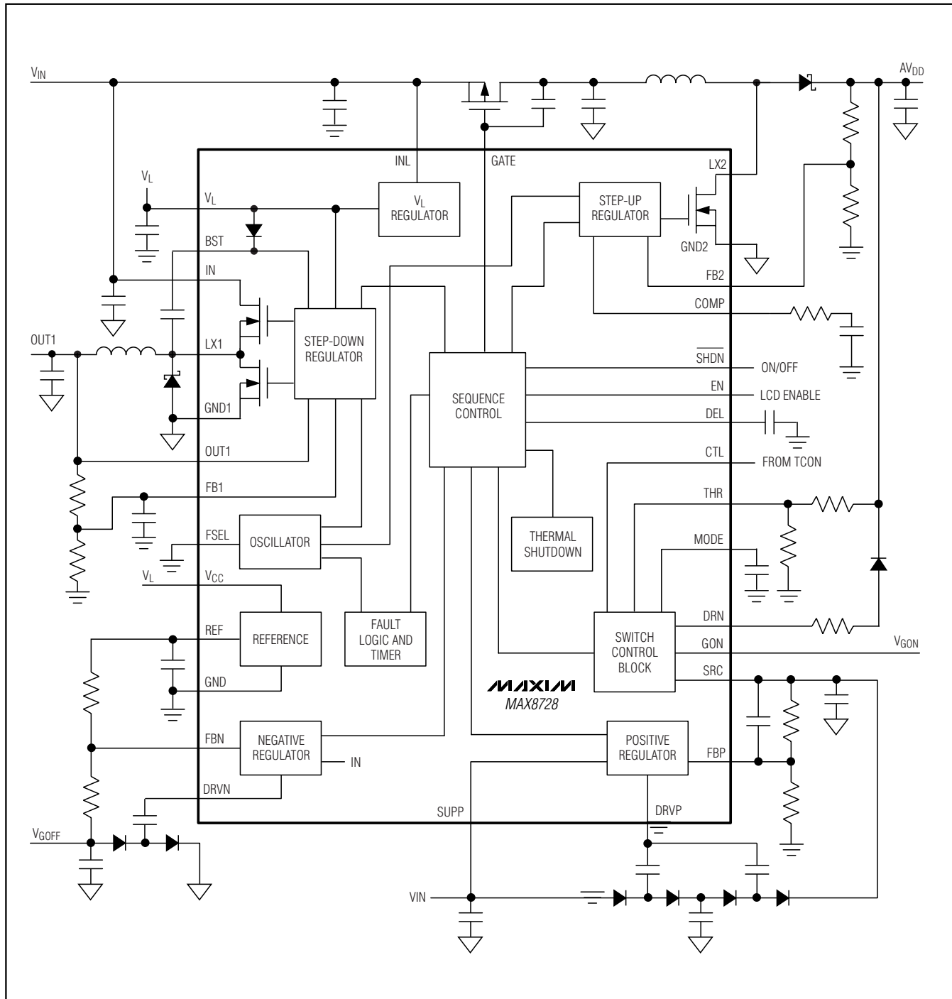
Figure 2. Functional Diagram
