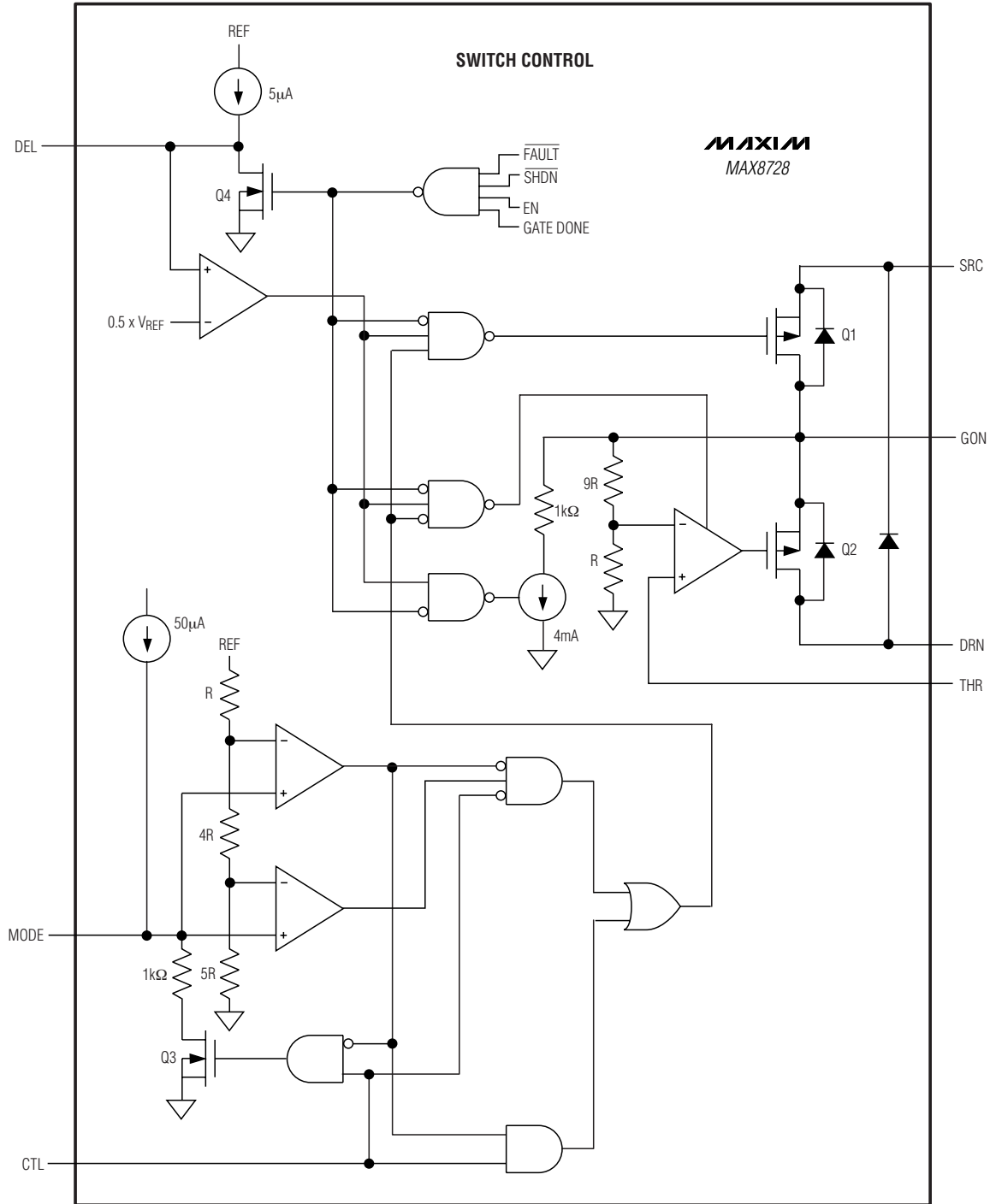
Figure 5. Switch-Control Functional Diagram
