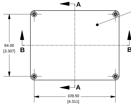
Top View of Assembly
