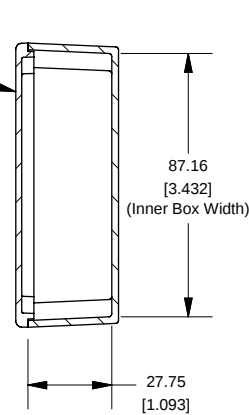
SECTION A-A End View of Assembly
