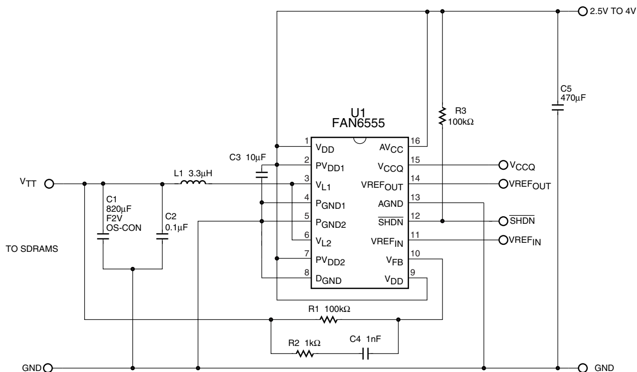
Figure 2. Alternate Application Circuit
