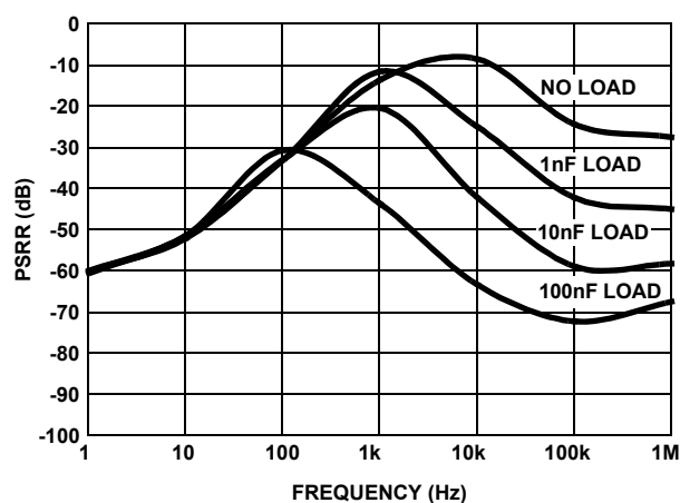
FIGURE 22. PSRR vs CAPACITIVE LOAD
