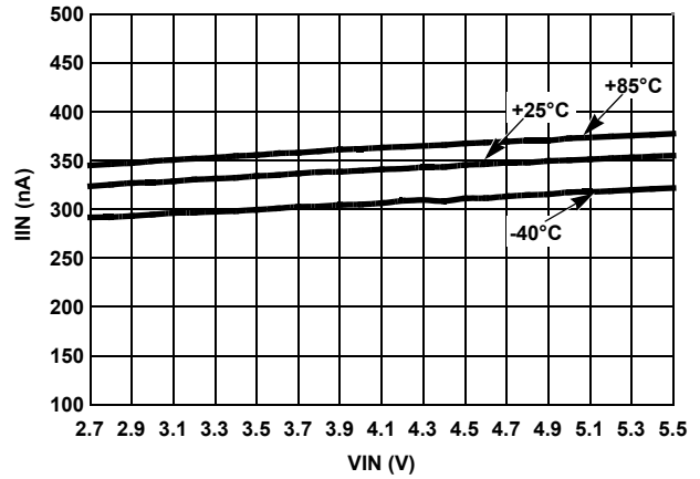
FIGURE 3. I_{IN} vs V_{IN} OVER-TEMPERATURE
