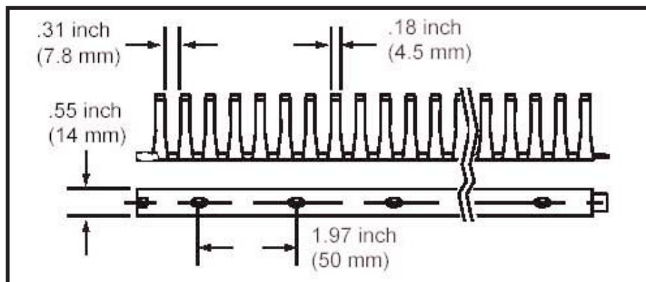
All other VK-FLEX side view
