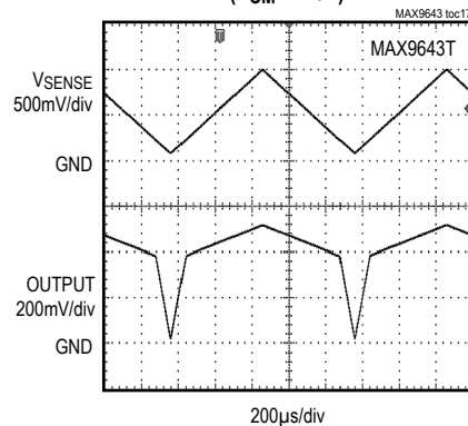
INPUT SENSE VOLTAGE SATURATION ( V_{CM} = 1.5V )
