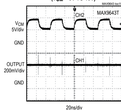
COMMON MODE ( V_{CM} = 0V TO 10V )
