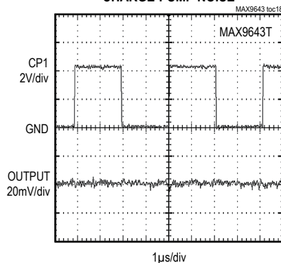
CHARGE-PUMP NOISE
