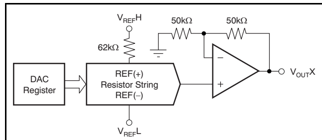
Figure 92. DAC8565 Architecture
