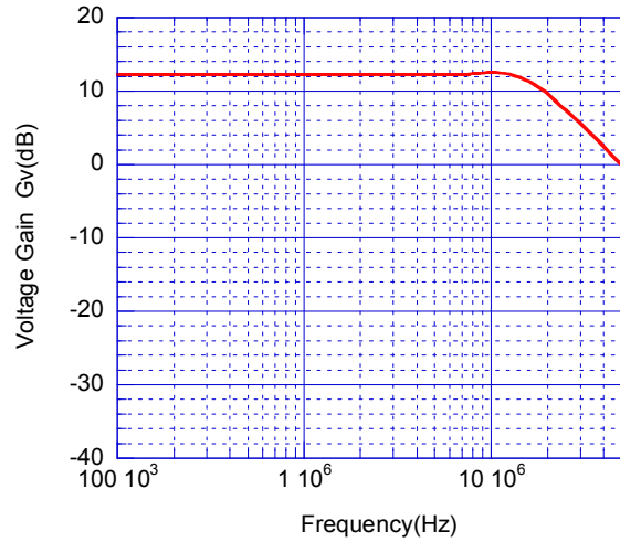
Voltage Gain vs. Frequency (Bias+Through Input)
