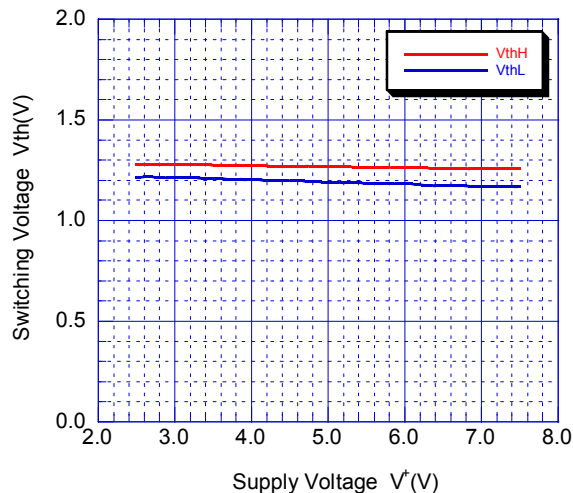
Switching Voltage vs. Supply Voltage
