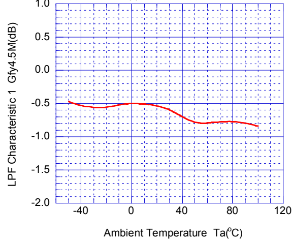
Low Pass Filter Characteristic 1 vs. Temperature (Clamp+LPF Type Input) 0.5Vpp, 4.5MHz/100kHz
