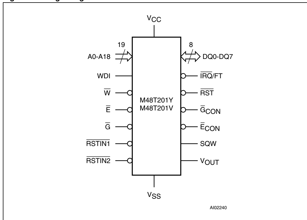
Figure 1. Logic diagram
