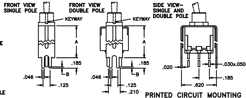
PRINTED CIRCUIT MOUNTING
