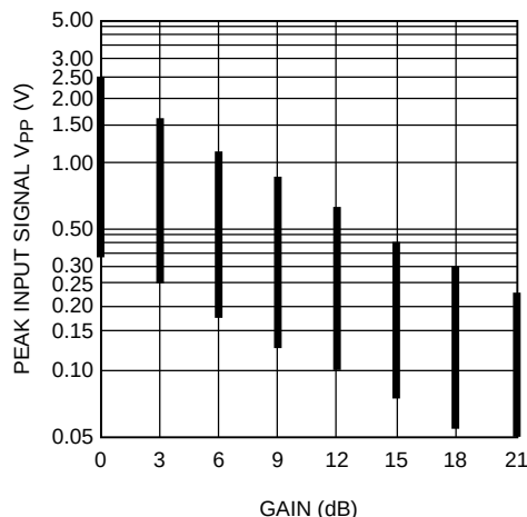
Figure 19. Peak Input Signal Level Range vs Gain Setting
