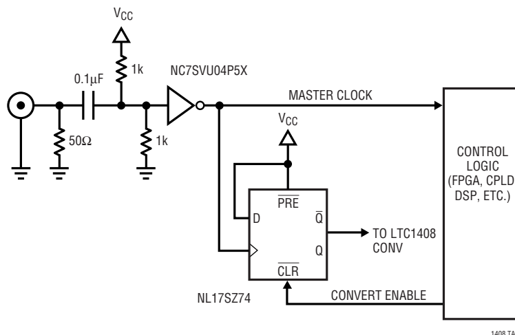
Clock Squaring/Level Shifting Circuit Allows Testing with RF Sine Generator. Convert Re-Timing Flip-Flop Preserves Low-Jitter Clock Timing
