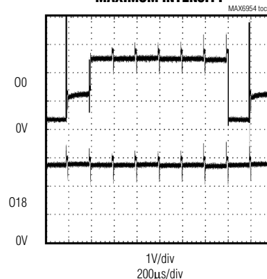
WAVEFORM AT PINS 00 AND 018, MAXIMUM INTENSITY
