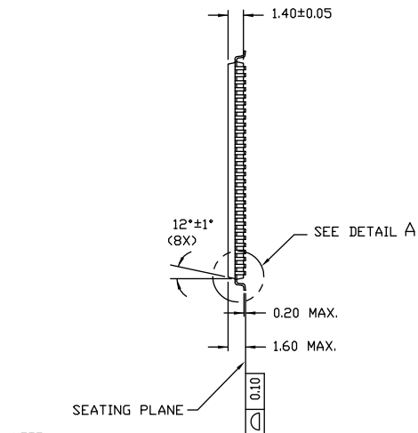
Figure 7. 100-pin TQFP (14 × 20 × 1.4 mm) A100RA Package Outline, 51-85050
