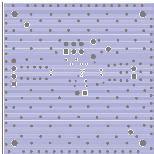
Figure 9. Bottom Layer
