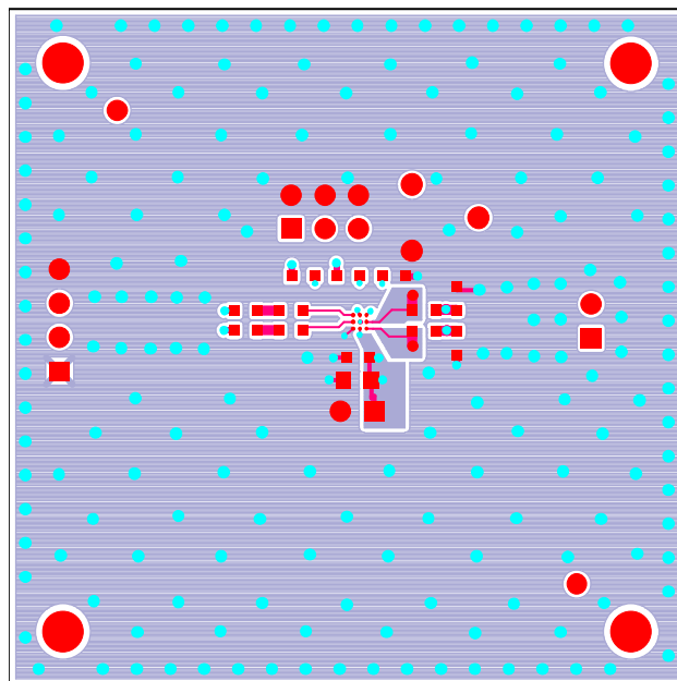
Figure 6. Top Layer
