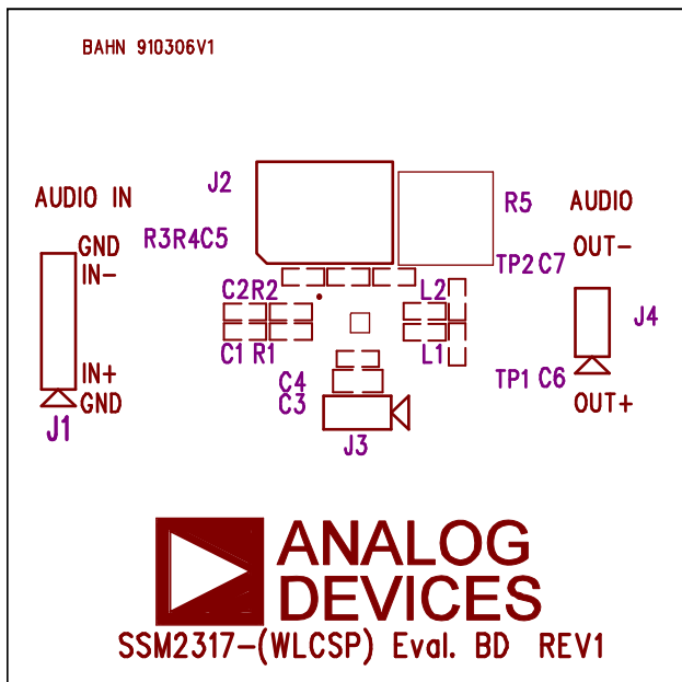
Figure 5. Top Silkscreen
