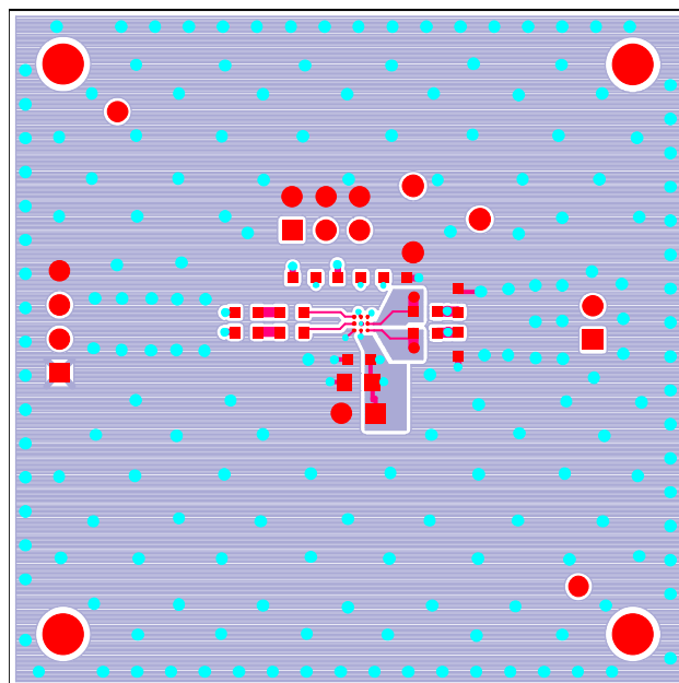
Figure 7. Layer 2 (Ground Plane)
