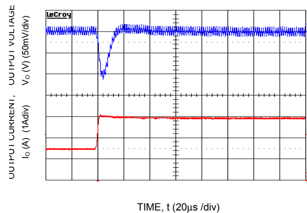
Figure 34. Transient Response to Dynamic Load Change from 50% to 100% at 12Vin, C_{out}=1x47\mu F , C_{Tune}=820pF & R_{Tune}=261
