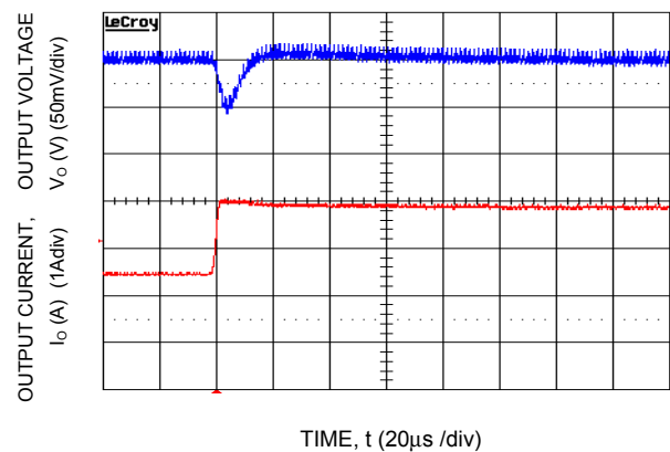
Figure 22. Transient Response to Dynamic Load Change from 50% to 100% at 12Vin, C_{out}=2x47\mu F , CTune-2700pF & RTune-261
