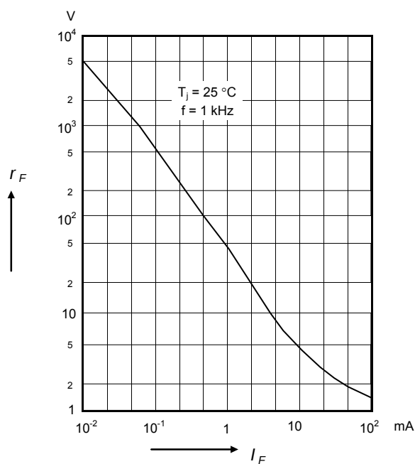
Dynamic forward resistance versus forward current
